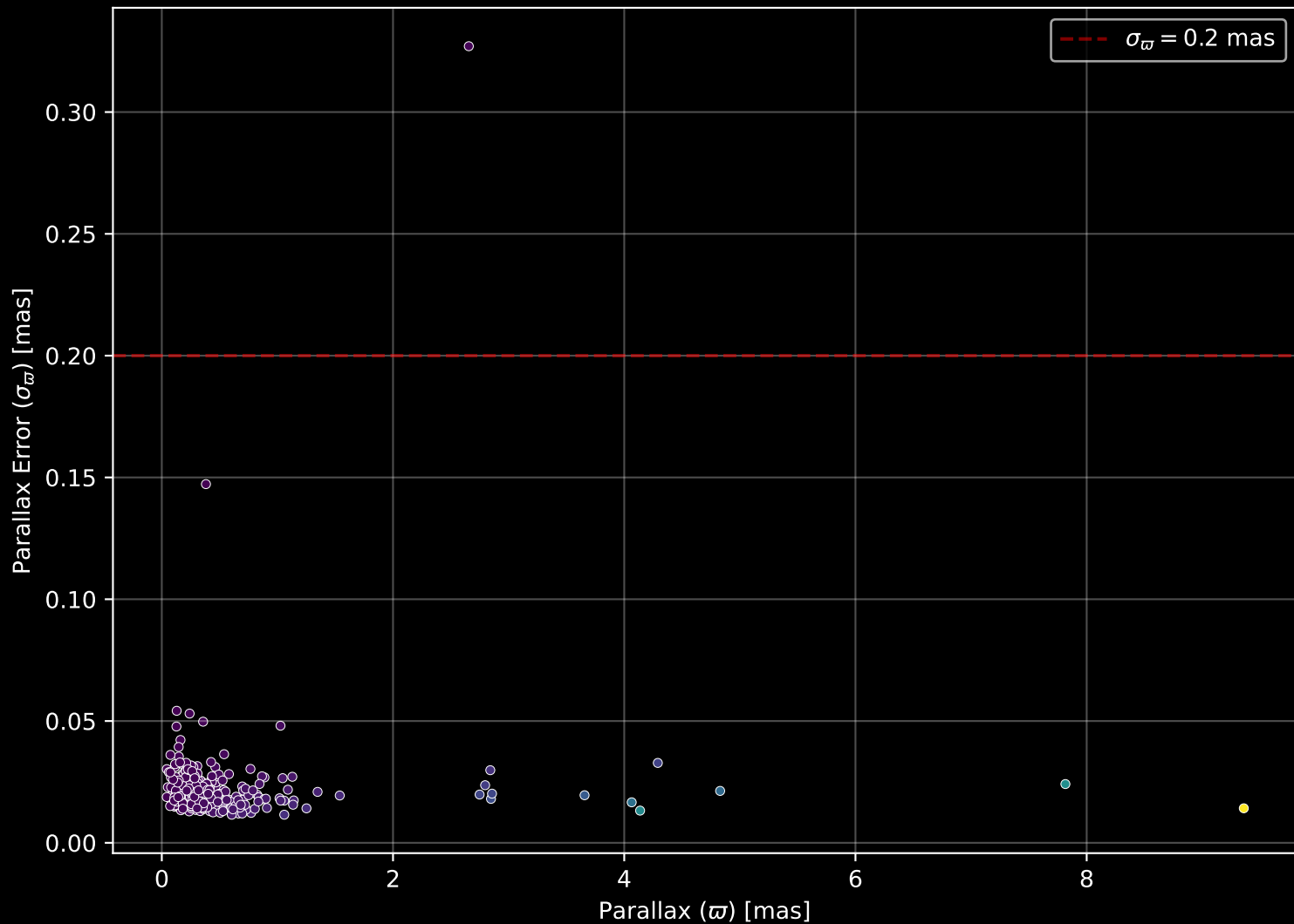
APOGEE DR17 Field: [COROT2] Parallax Quality (n= 380)
