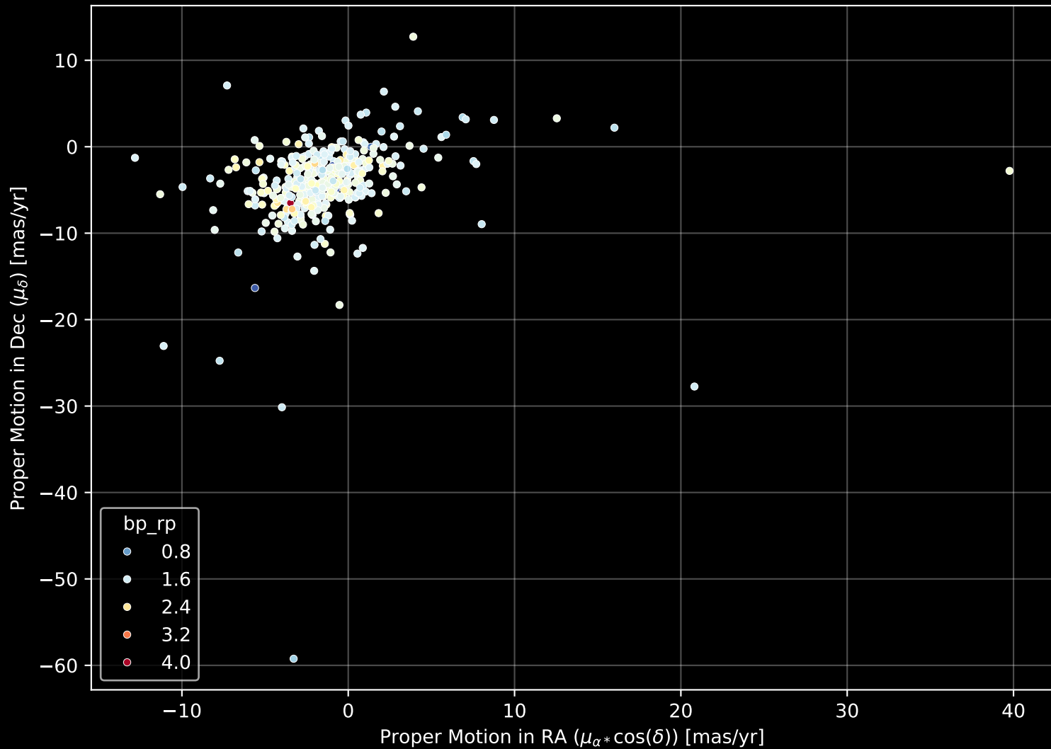
APOGEE DR17 Field: [COROT2] Proper Motion Diagram (n= 380)
