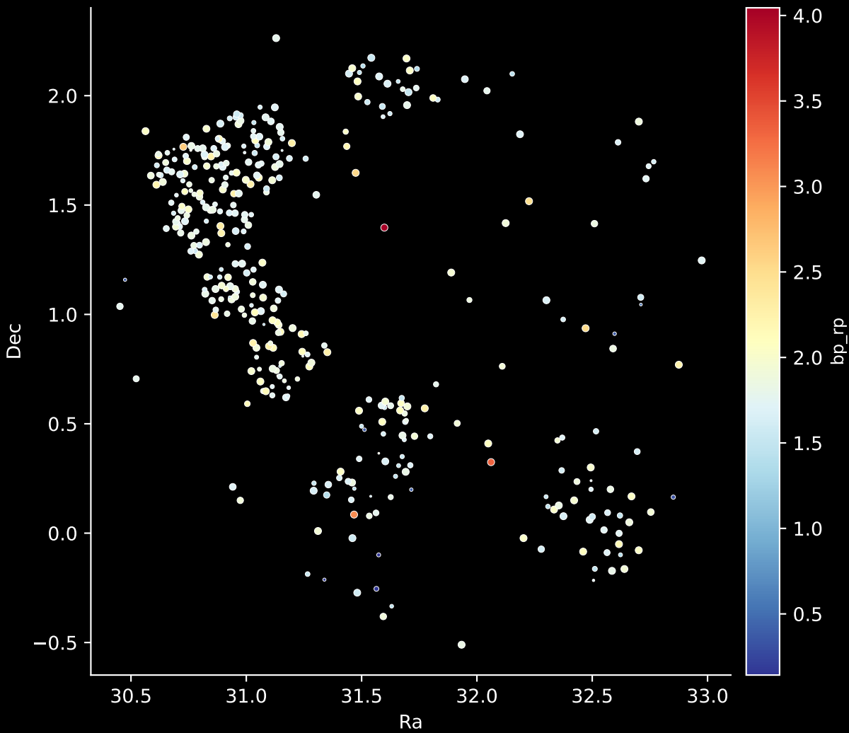
APOGEE DR17 Field: [COROT2] Stars: 380
