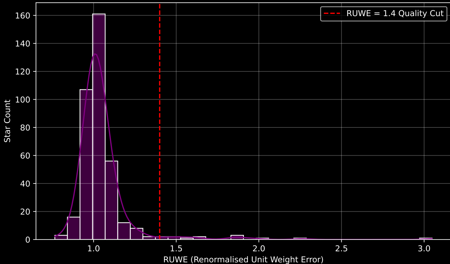
GAPOGEE DR17 Field [COROT2] RUWE Distribution (n= 378)
