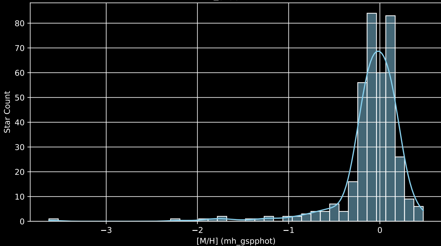
APOGEE DR17 Field: [COROT2 [M/H] (mh_gspphot) (n= 376)
