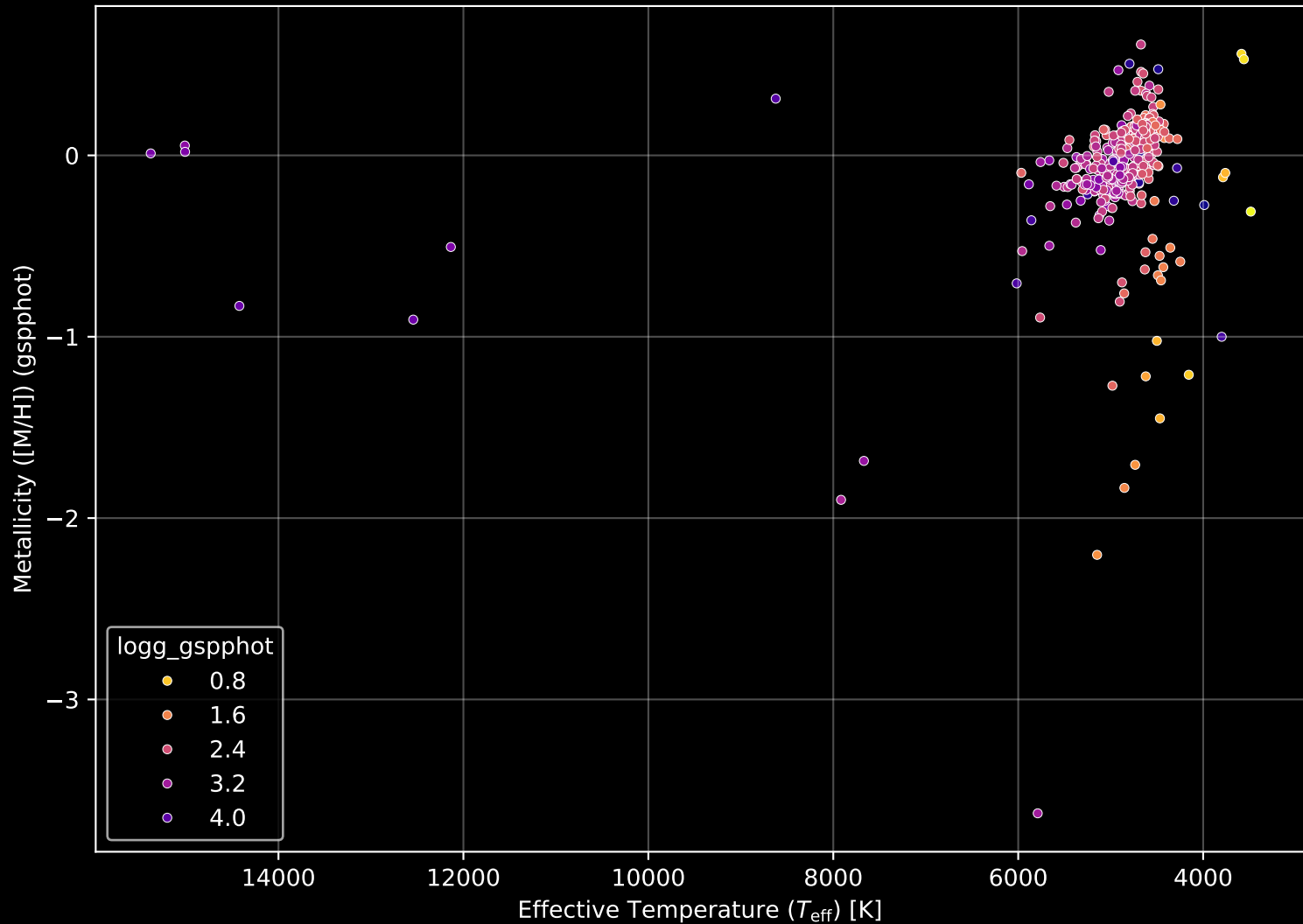
APOGEE DR17 Field: [COROT2] Stellar Population Parameters (n= 380)
