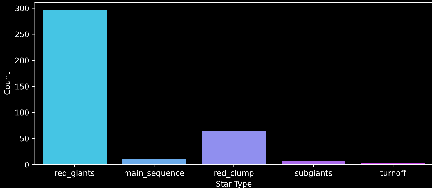
APOGEE DR17 Field: [COROT2] Count plot of Star Type
